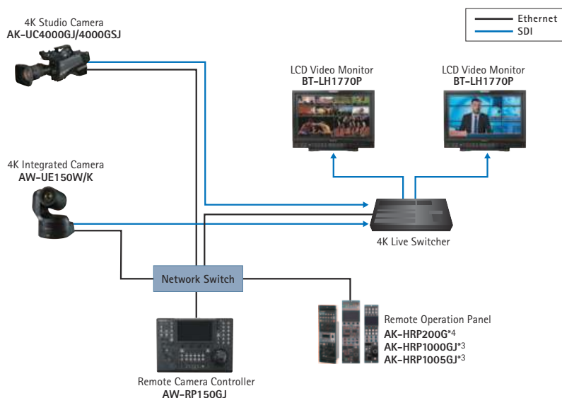
■ Example of connection using RTMP
