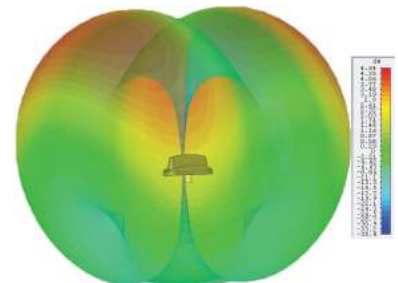
3D Gain Plot Top (2600MHz)
