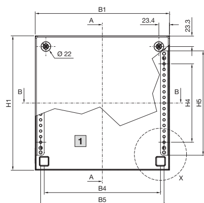
3 Internal view
