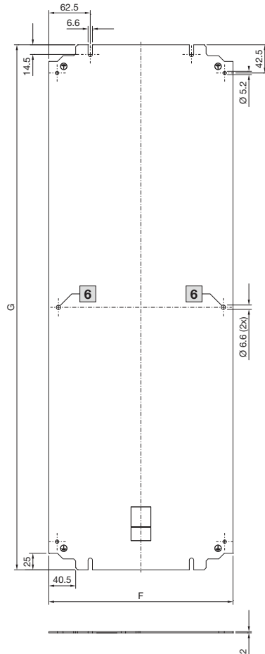
Mounting plate
