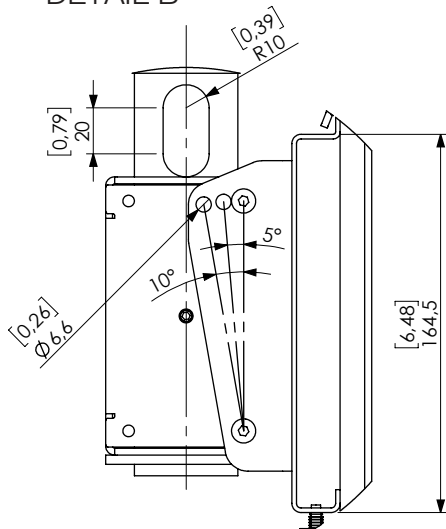
DETAIL B
